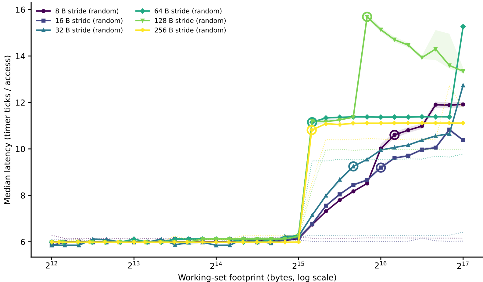
upgrade: line-size family of curves (dependent pointer chase) (Phase I timing-only, level boundary=32768B window=[4096,131072])
