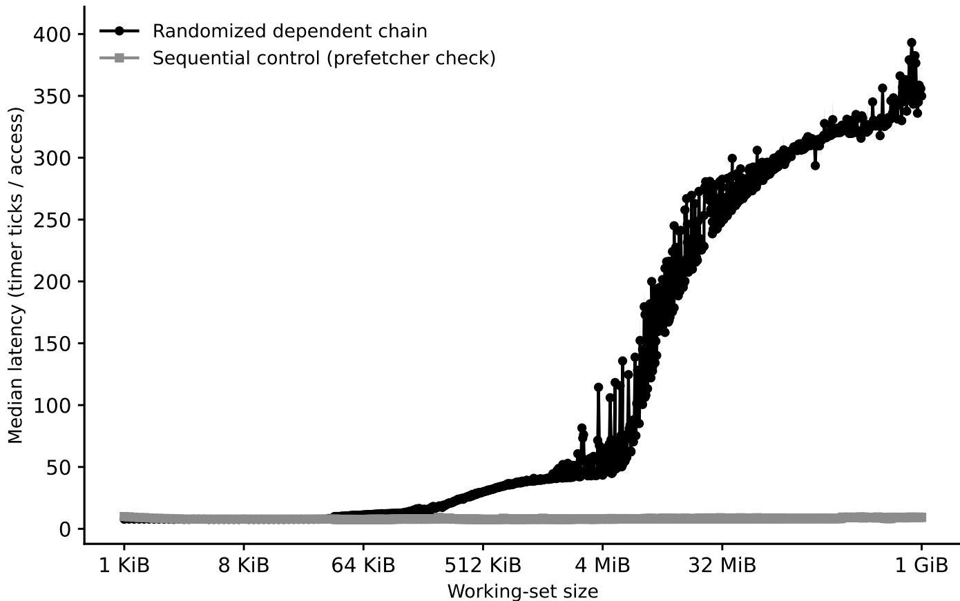
charnwood: capacity sweep (dependent pointer chase)
