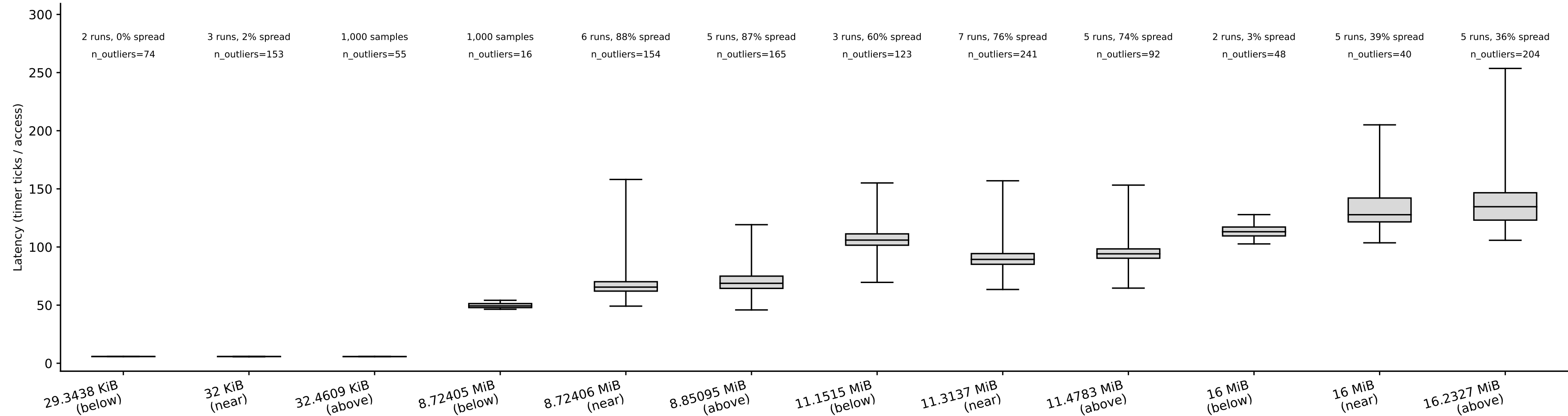
crux: capacity box plots, random pattern (whiskers = p5/p95) tested boundaries: 32 KiB, 8.72406 MiB, 11.3137 MiB, 16 MiB
