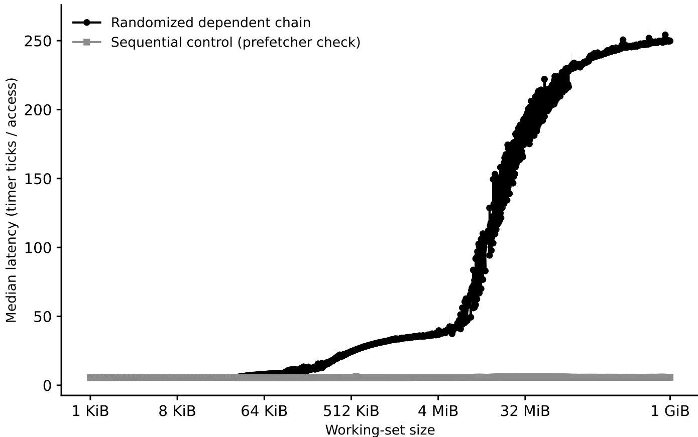
crux: capacity sweep (dependent pointer chase)
