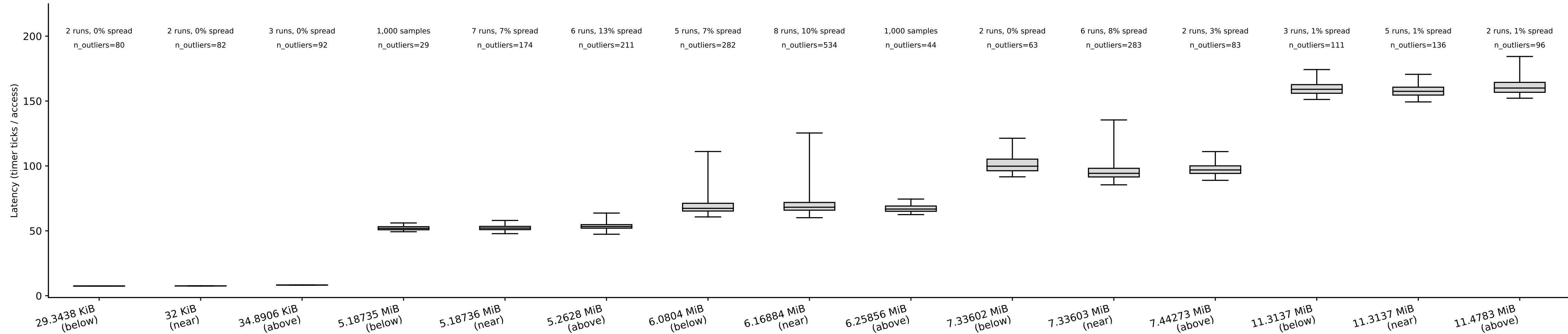
ookay: capacity box plots, random pattern (whiskers = p5/p95) tested boundaries: 32 KiB, 5.18736 MiB, 6.16884 MiB, 7.33603 MiB, 11.3137 MiB
