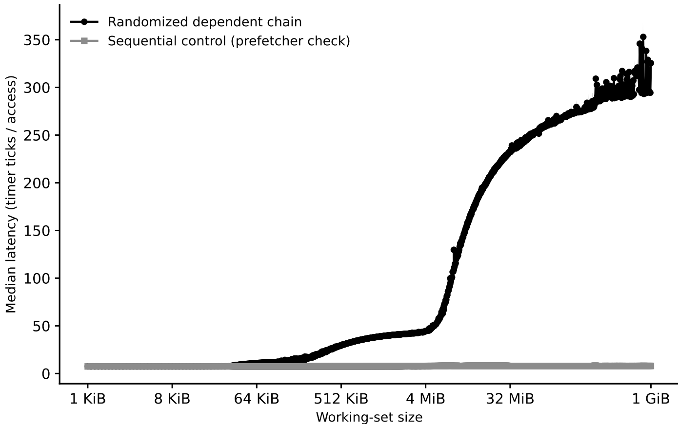
ookay: capacity sweep (dependent pointer chase)
