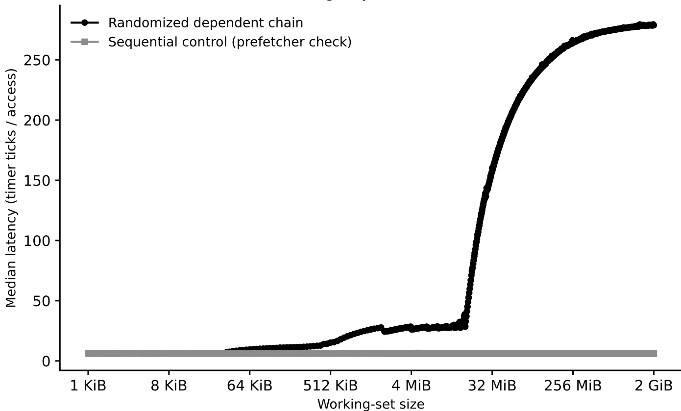
skylark: capacity sweep (dependent pointer chase) (Phase I timing-only, extended to 2 GiB)
