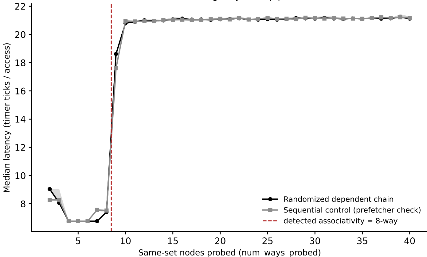
hazel_cascadelake: associativity sweep, L1 (stride=32 KiB) (Phase I timing-only, auto pipeline)
