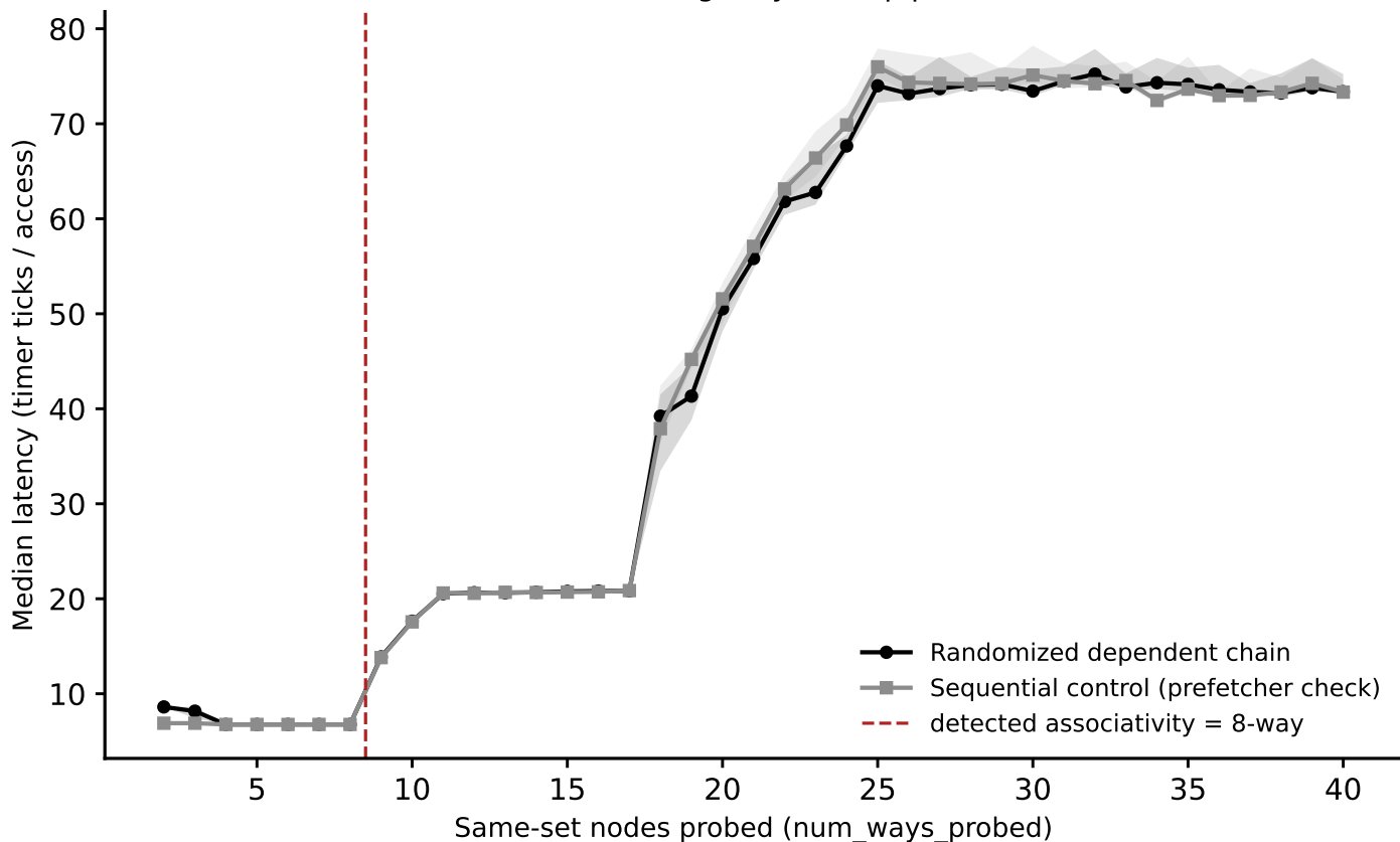
hazel_cascadelake: associativity sweep, L3_LLC (stride=16 MiB) (Phase I timing-only, auto pipeline)
