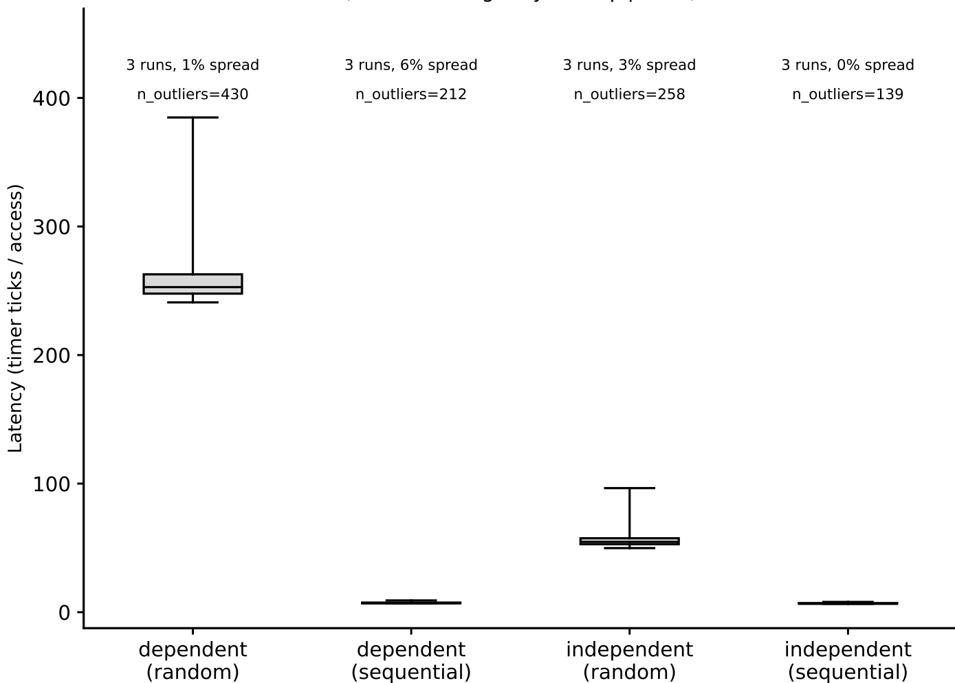
hazel_cascadelake: hit-latency box plots, DRAM (footprint=512 MiB) (Phase I timing-only, auto pipeline)
