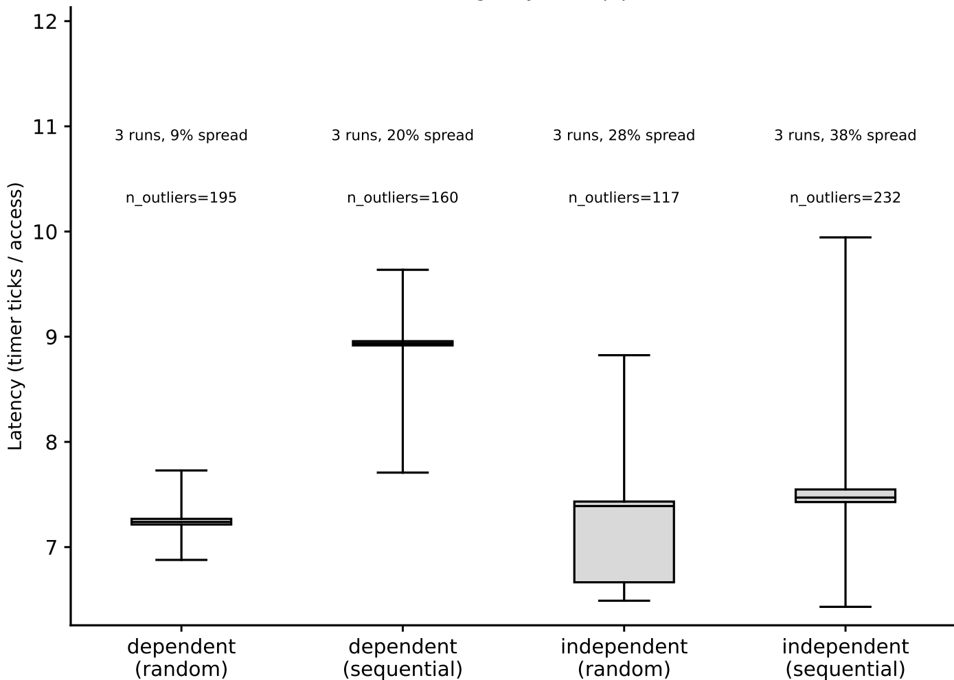
hazel_cascadelake: hit-latency box plots, L1 (footprint=32 KiB) (Phase I timing-only, auto pipeline)
