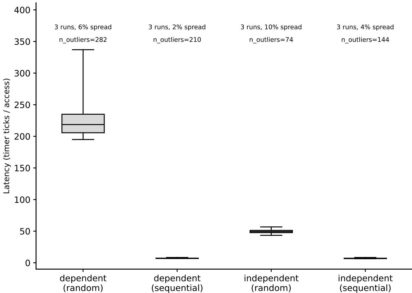
hazel_cascadelake: hit-latency box plots, LLC (footprint=16 MiB) (Phase I timing-only, auto pipeline)
