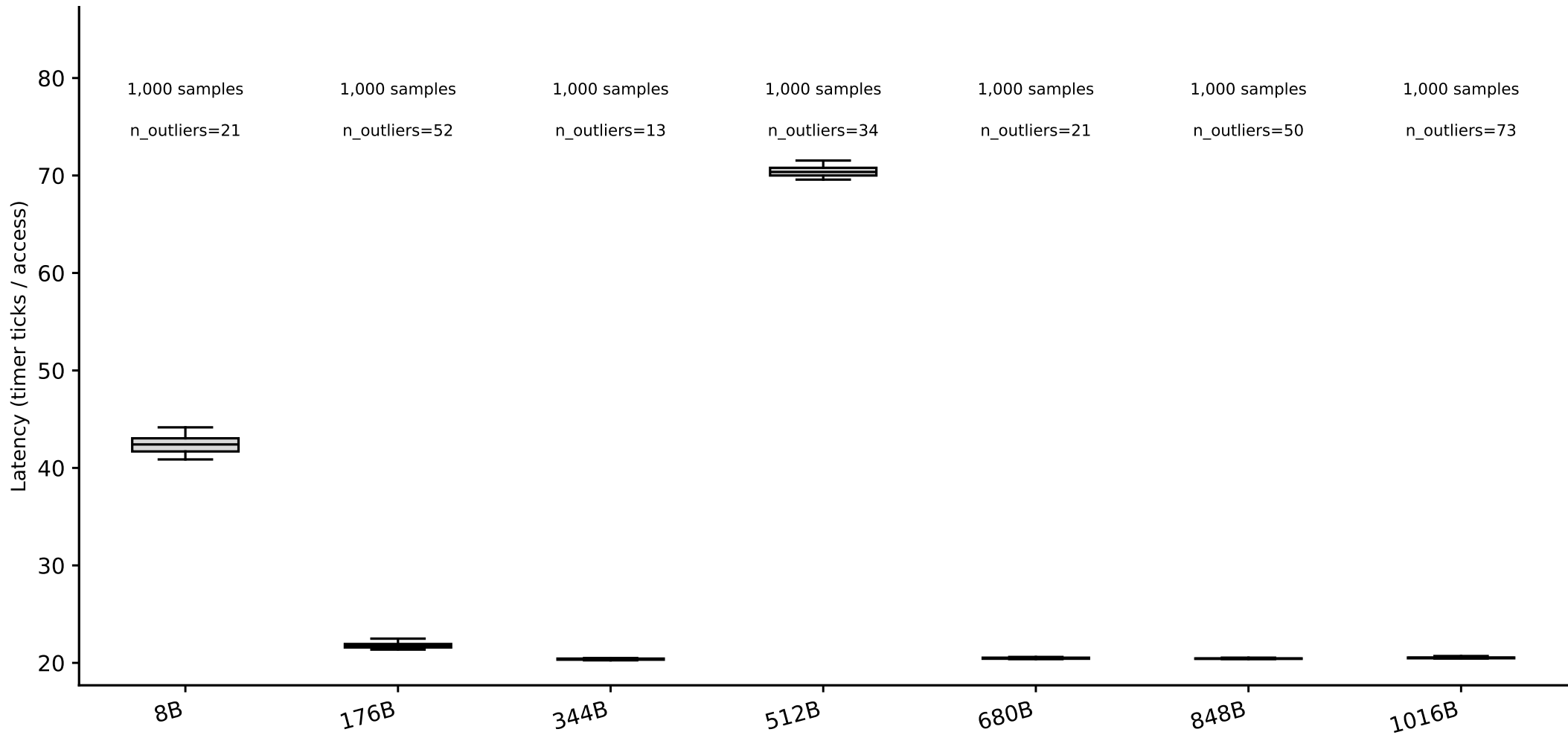
hazel_cascadelake: line-size box plots, random pattern (whiskers = p5/p95) (Phase I timing-only, level boundary=1048576B, single-curve method)
