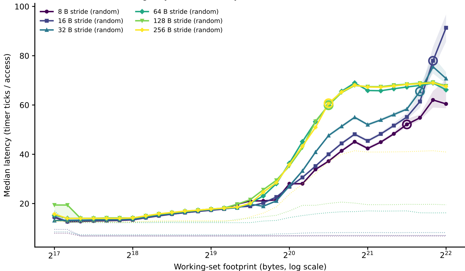
hazel_cascadelake: line-size family of curves (dependent pointer chase) (Phase I timing-only, level boundary=1048576B window=[131072,4194304])
