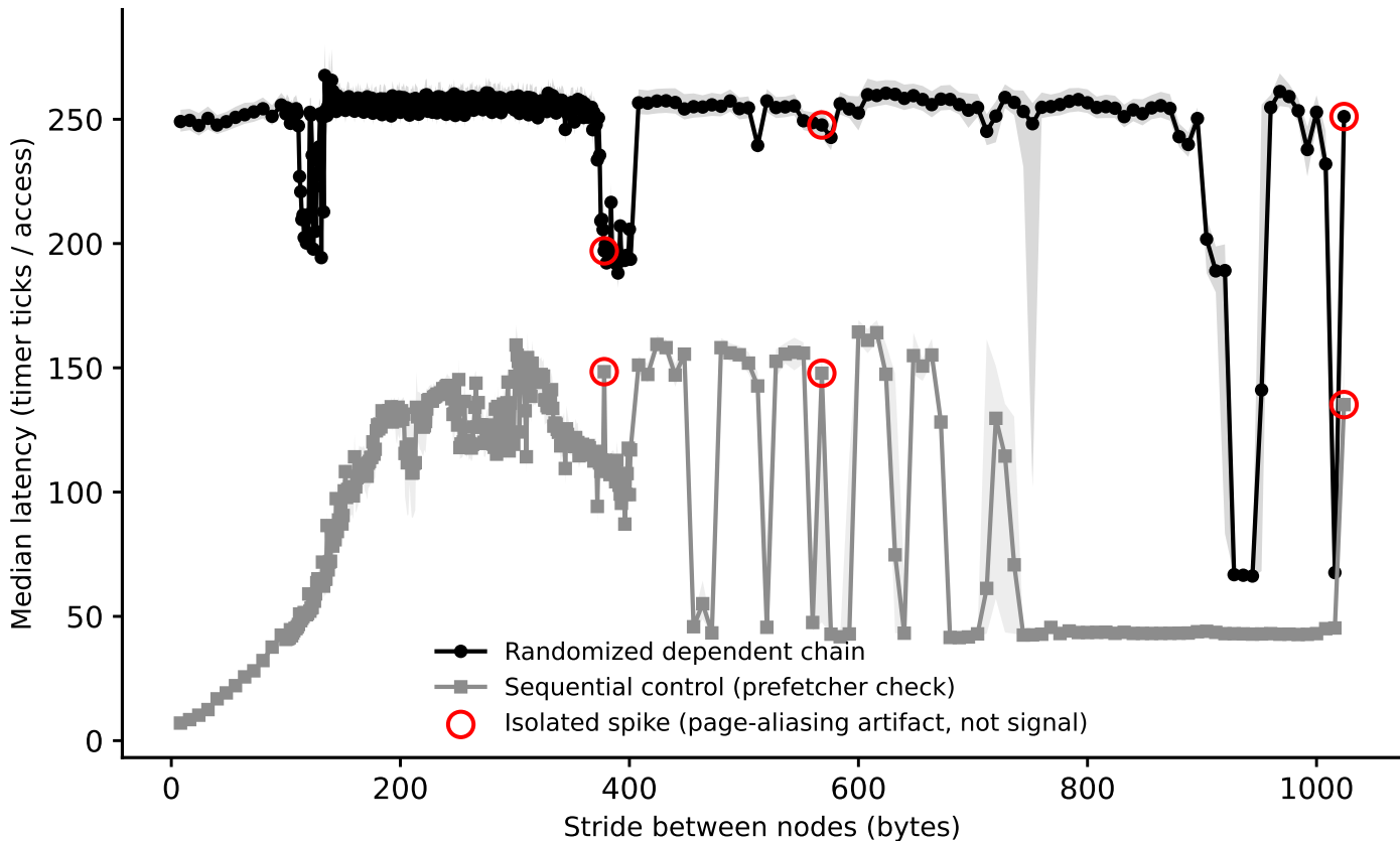
hazel_cascadelake: line-size sweep (dependent pointer chase), footprint=32 MiB (Phase I timing-only, level boundary=16777216B, single-curve method)
