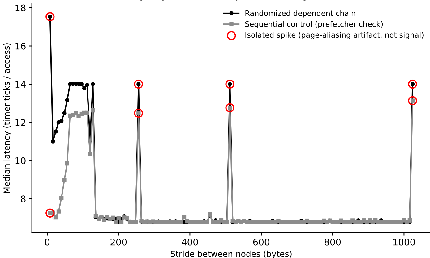
hazel_cascadelake: line-size sweep (dependent pointer chase), footprint=64 KiB (Phase I timing-only, level boundary=32768B, single-curve method)
