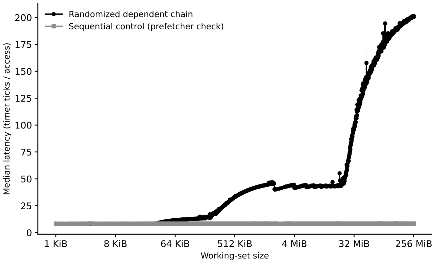
hazel_haswell: capacity sweep (dependent pointer chase) (Phase I timing-only, auto pipeline)
