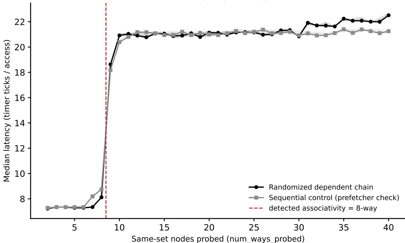
ookay: associativity sweep, L1 (stride=32 KiB) (Phase I timing-only, auto pipeline)
