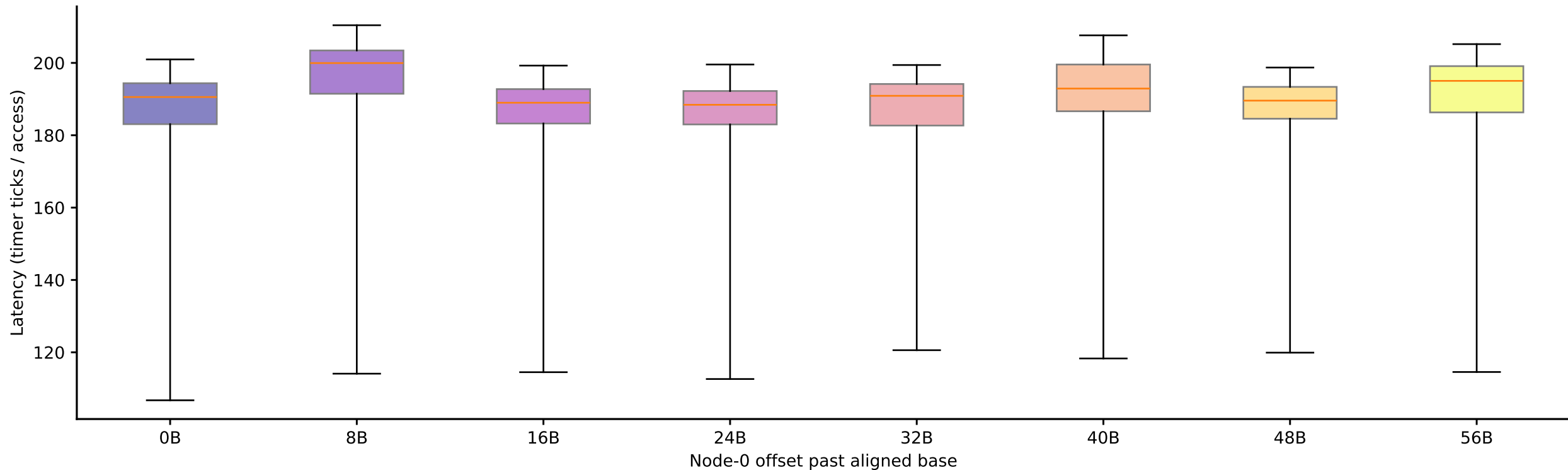
hazel_haswell: candidate stride 64 B at footprint 38.0976 MiB, by offset (Phase I timing-only, level boundary=25165824B, step-4 alignment refinement)
