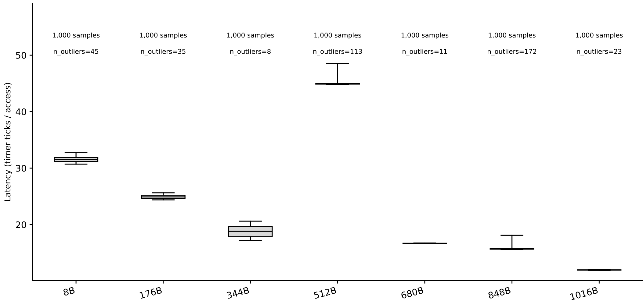
hazel_haswell: line-size box plots, random pattern (whiskers = p5/p95) (Phase I timing-only, level boundary=262144B, single-curve method)
