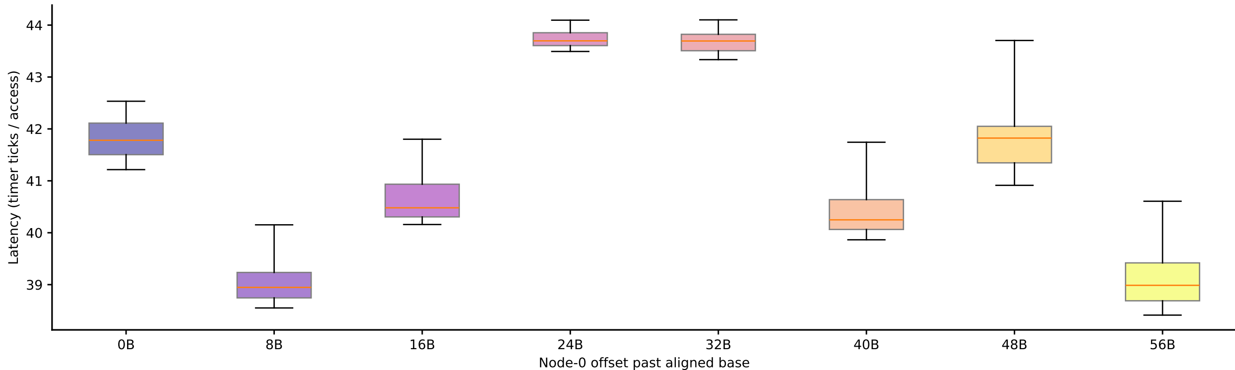
hazel_haswell: candidate stride 64 B at footprint 362 KiB, by offset (Phase I timing-only, level boundary=262144B, step-4 alignment refinement)
