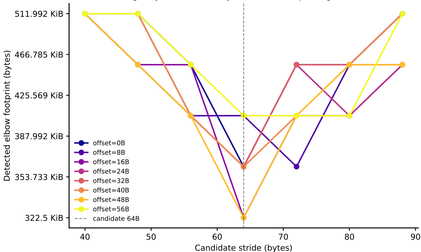
hazel_haswell: line-size elbow vs. stride, by node-0 offset (Phase I timing-only, level boundary=262144B, step-4 alignment refinement)
