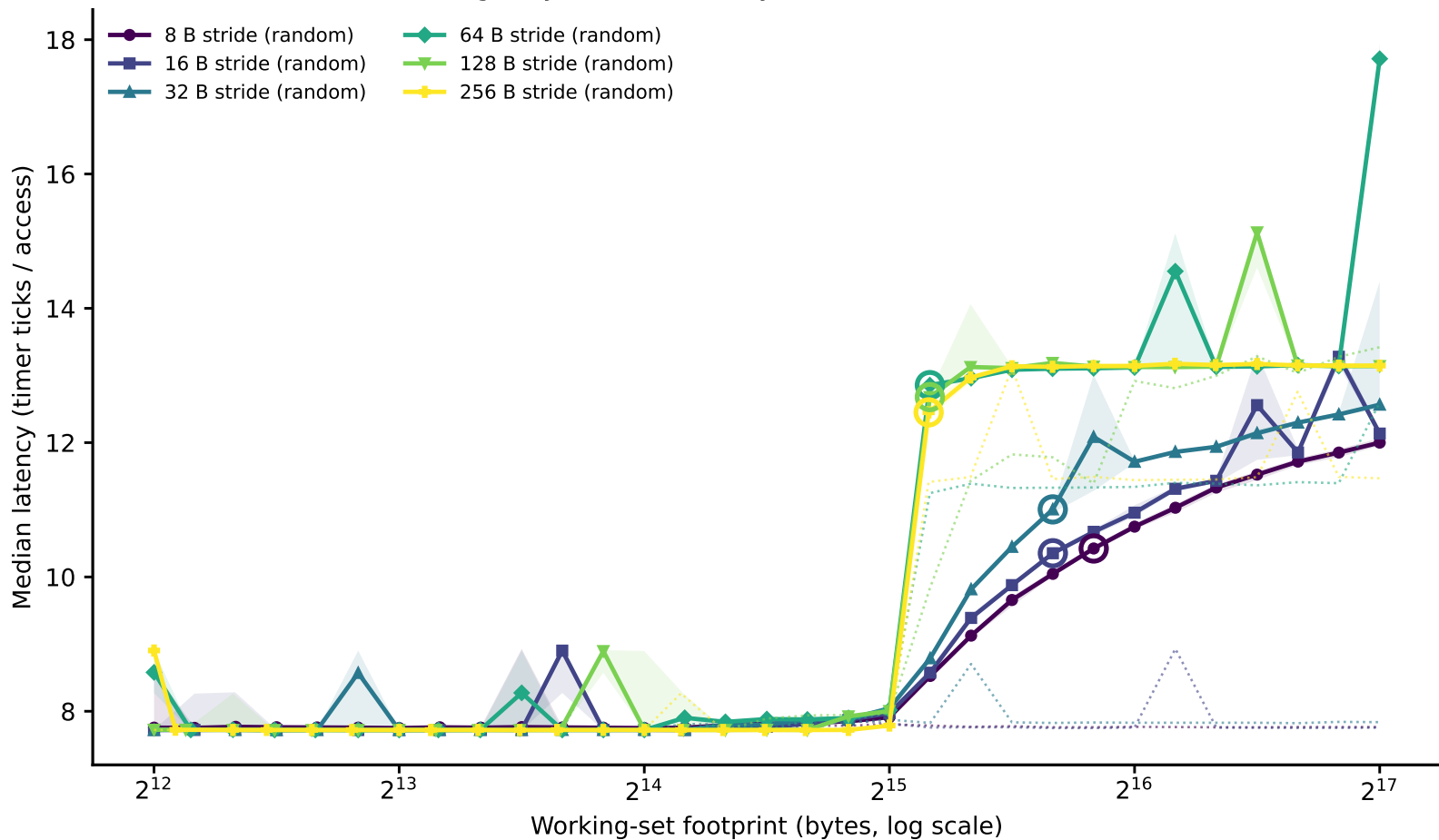
hazel_haswell: line-size family of curves (dependent pointer chase) (Phase I timing-only, level boundary=32768B window=[4096,131072])
