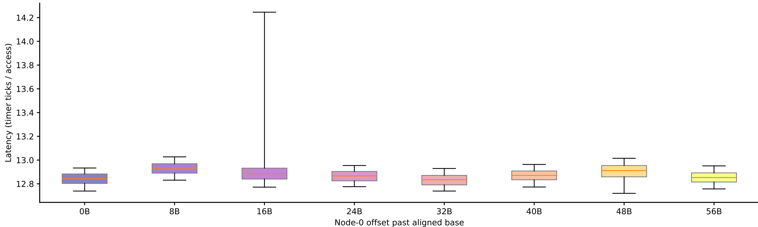
hazel_haswell: candidate stride 64 B at footprint 35.875 KiB, by offset (Phase I timing-only, level boundary=32768B, step-4 alignment refinement)
