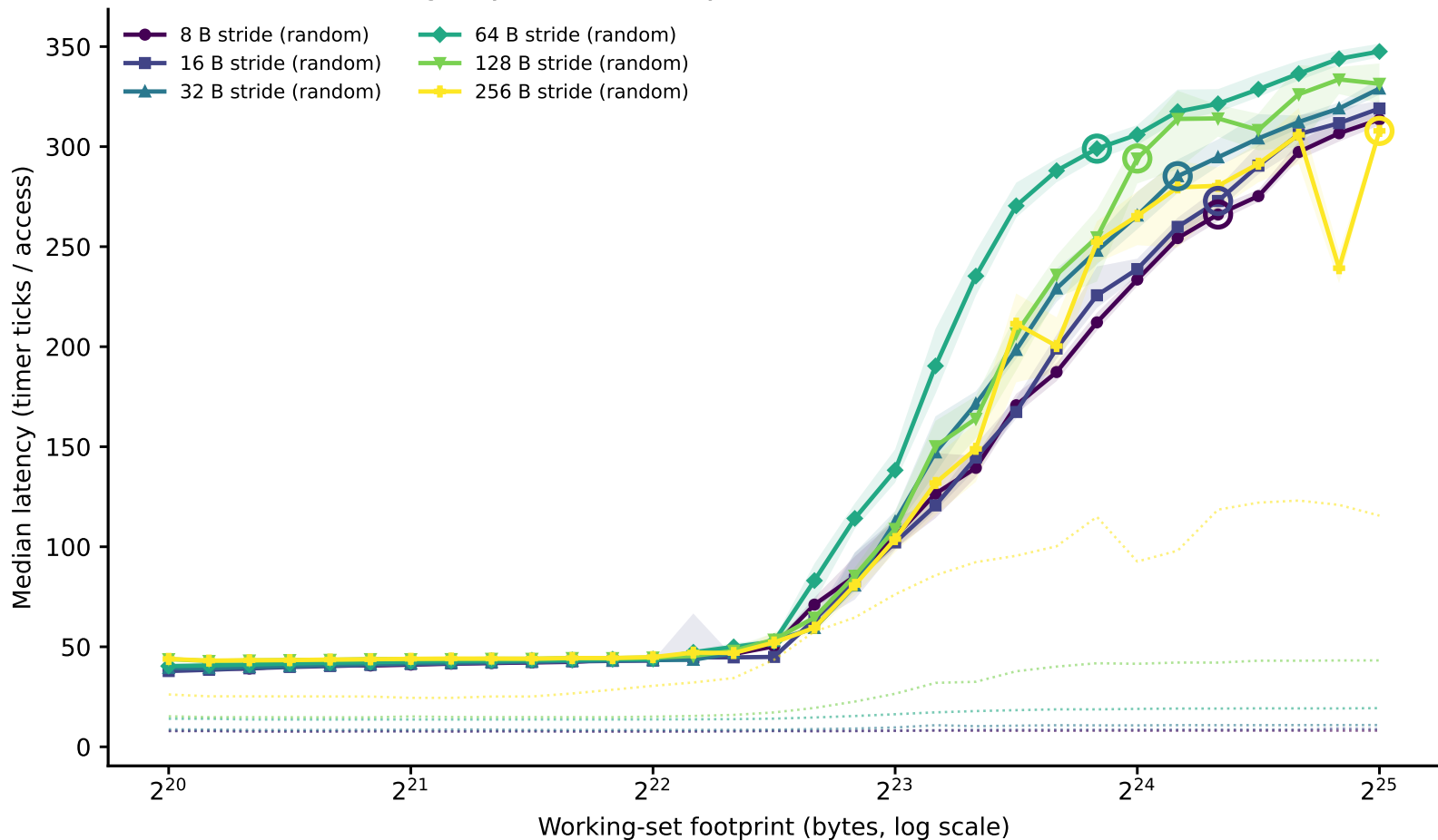
charnwood: line-size family of curves (dependent pointer chase) (Phase I timing-only, level boundary=8388608B window=[1048576,33554432])
