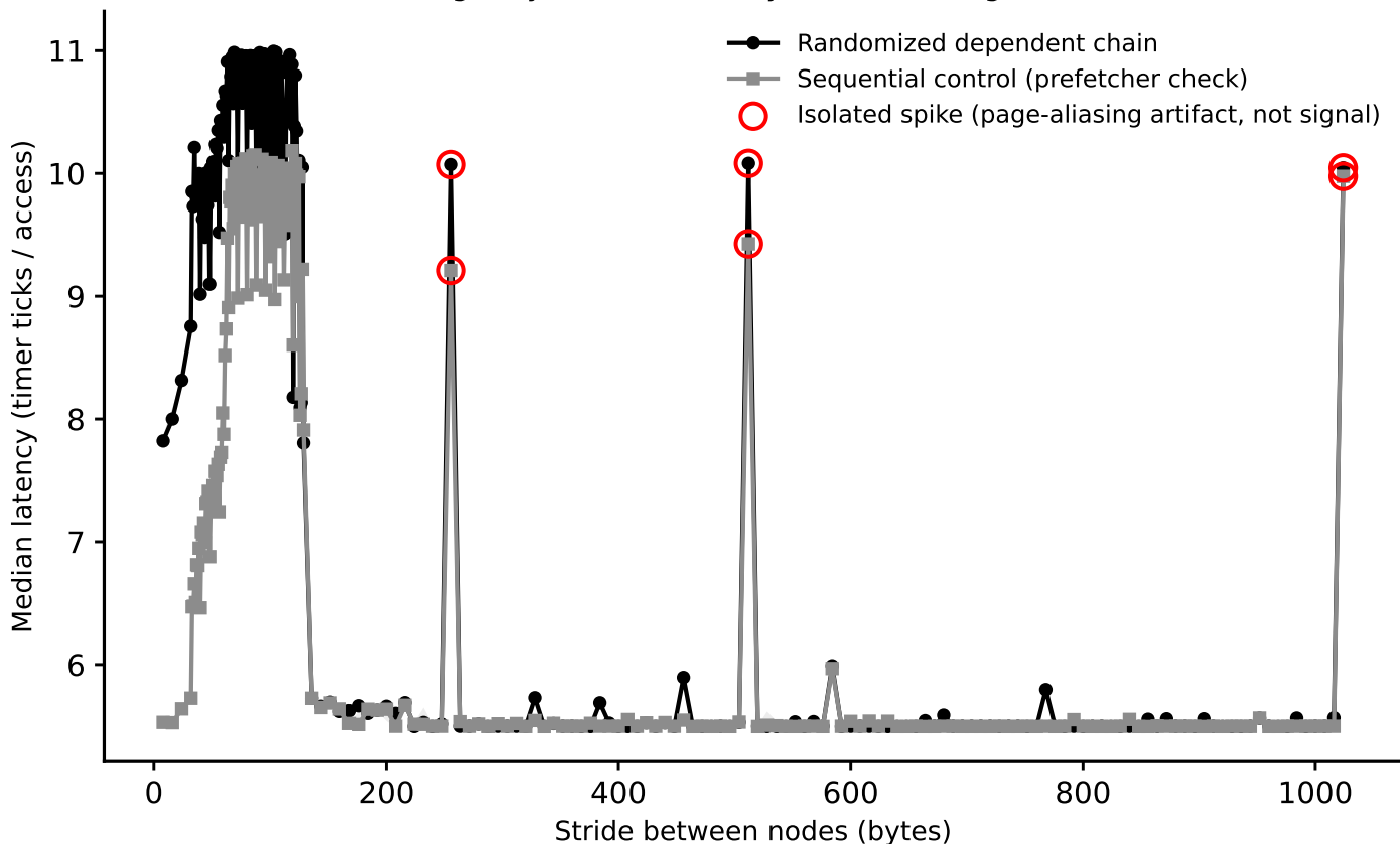
crux: line-size sweep (dependent pointer chase), footprint=64 KiB (Phase I timing-only, level boundary=32768B, single-curve method)
