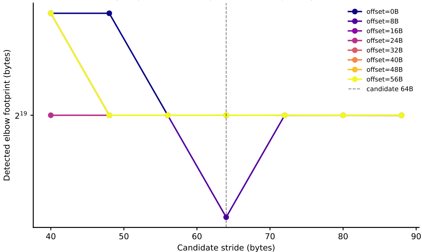
ookay: line-size elbow vs. stride, by node-0 offset (Phase I timing-only, level boundary=262144B, step-4 alignment refinement)
