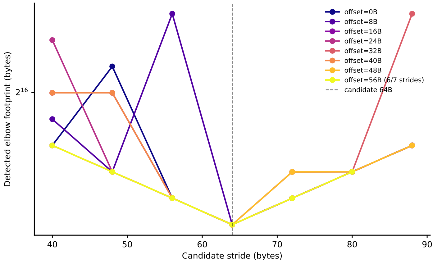
upgrade: line-size elbow vs. stride, by node-0 offset (Phase I timing-only, level boundary=32768B, step-4 alignment refinement)
