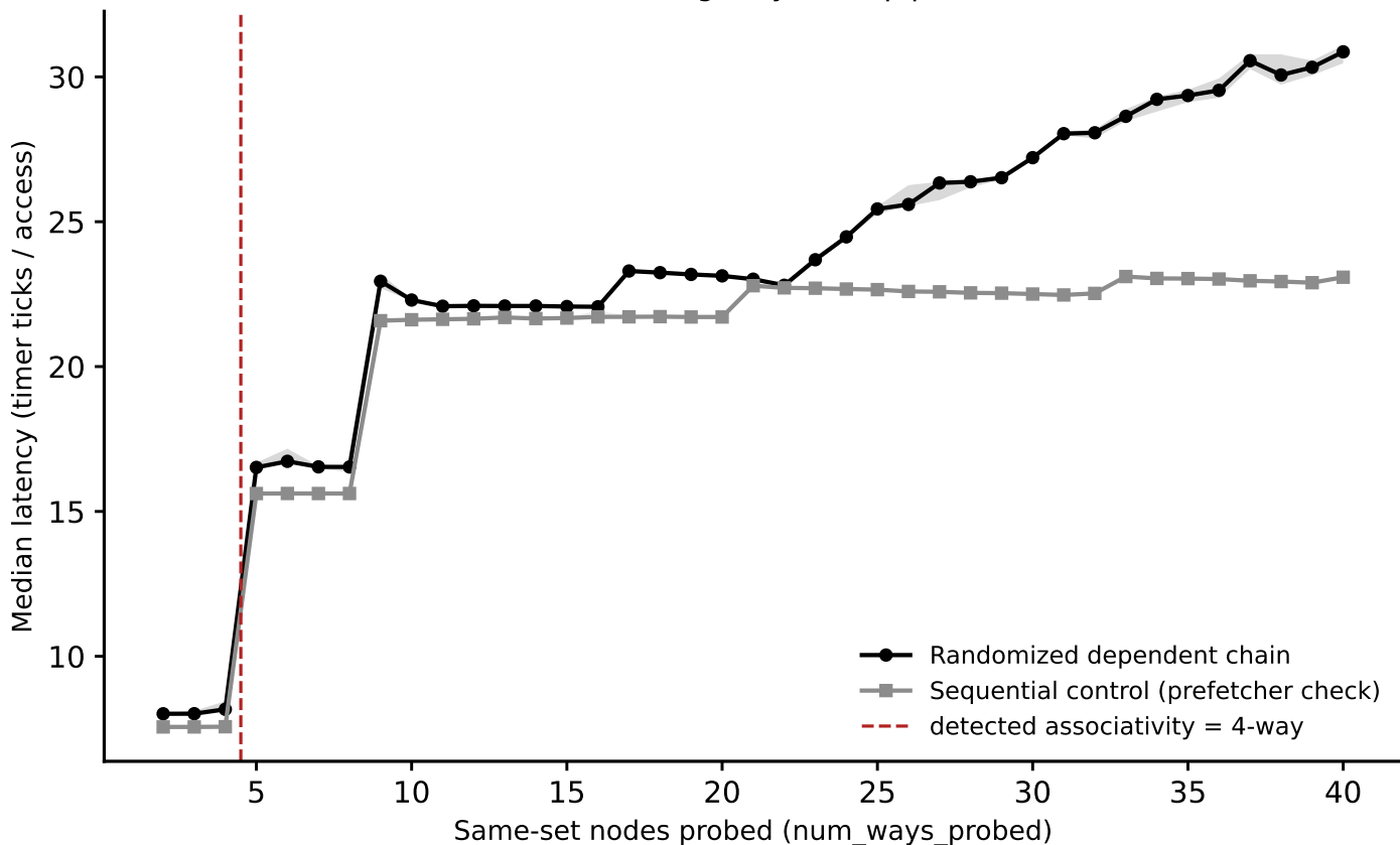
charnwood: associativity sweep, L2 (stride=256 KiB) (Phase I timing-only, auto pipeline)
