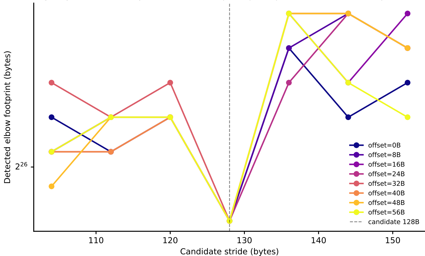
thunderbird: line-size elbow vs. stride, by node-0 offset base I timing-only, level boundary=31457280B, step-4 repro repeat seed=12346, compare vs seed
