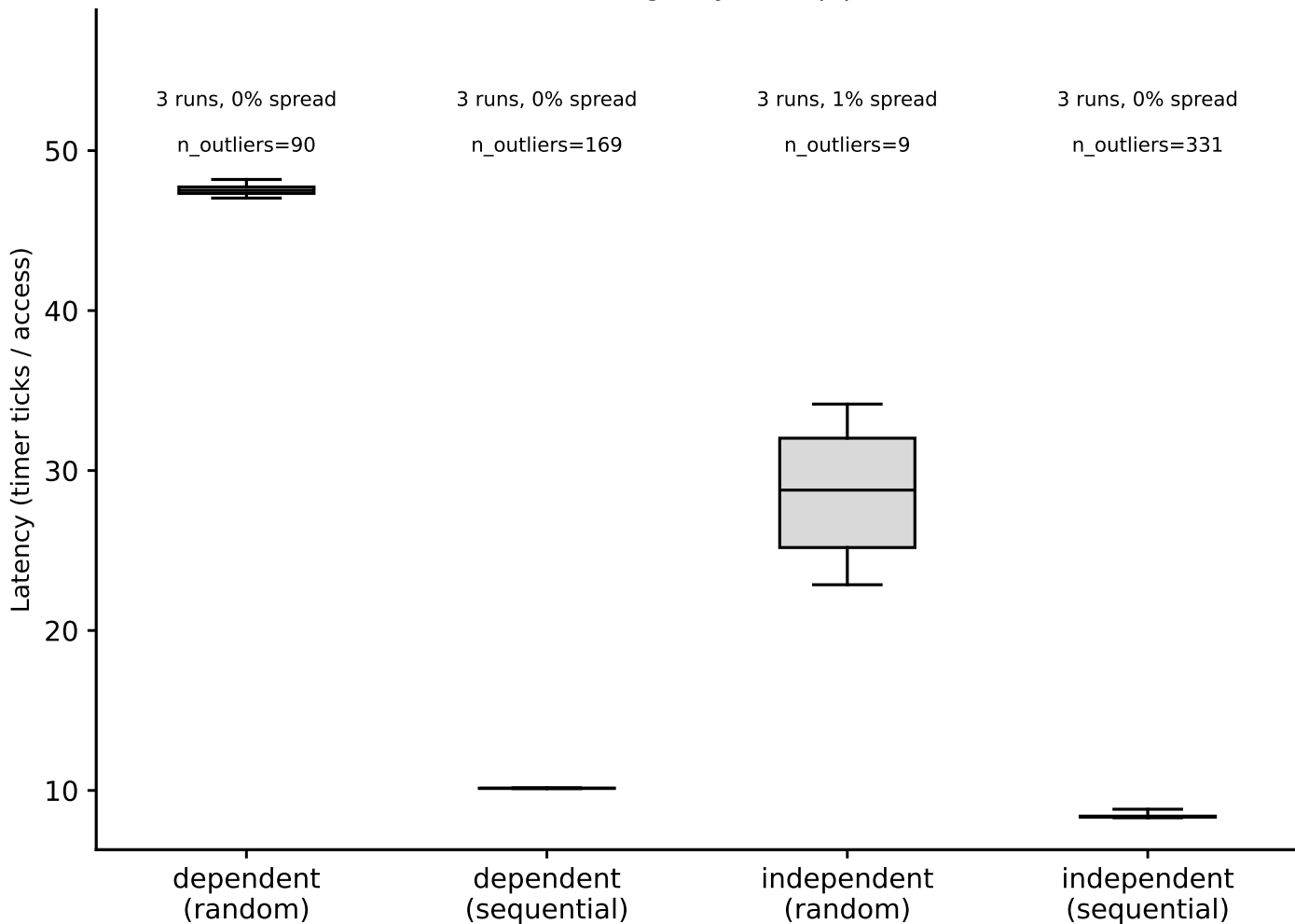
hazel_broadwell: hit-latency box plots, LLC (footprint=24.6754 MiB) (Phase I timing-only, auto pipeline)
