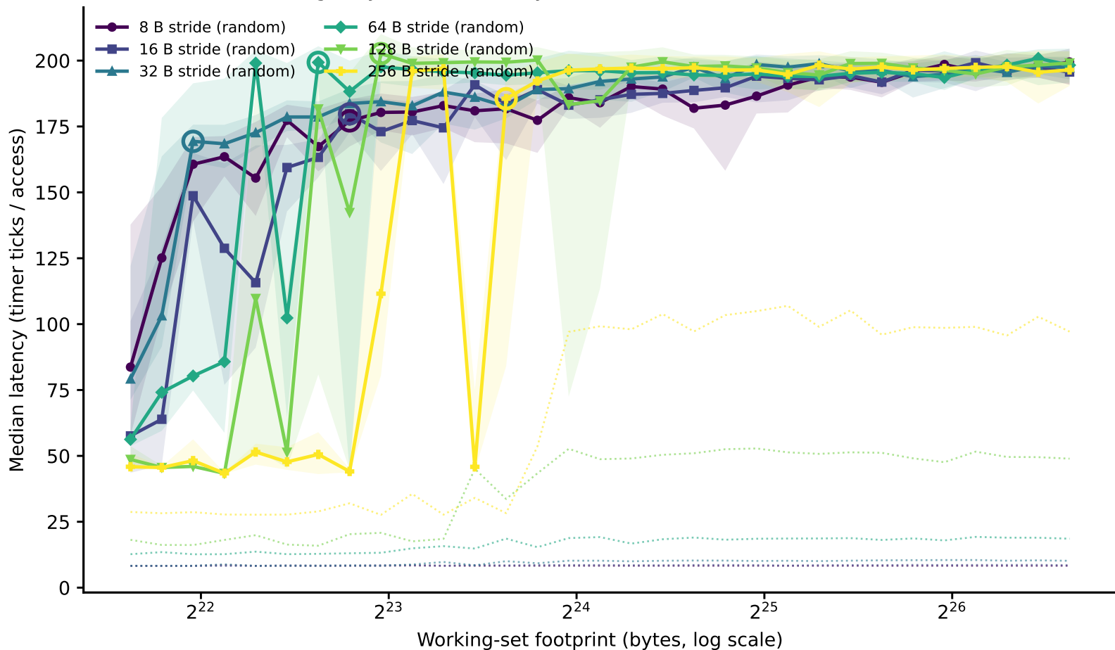
hazel_broadwell: line-size family of curves (dependent pointer chase) (Phase I timing-only, level boundary=25874000B window=[3234250,103496000])
