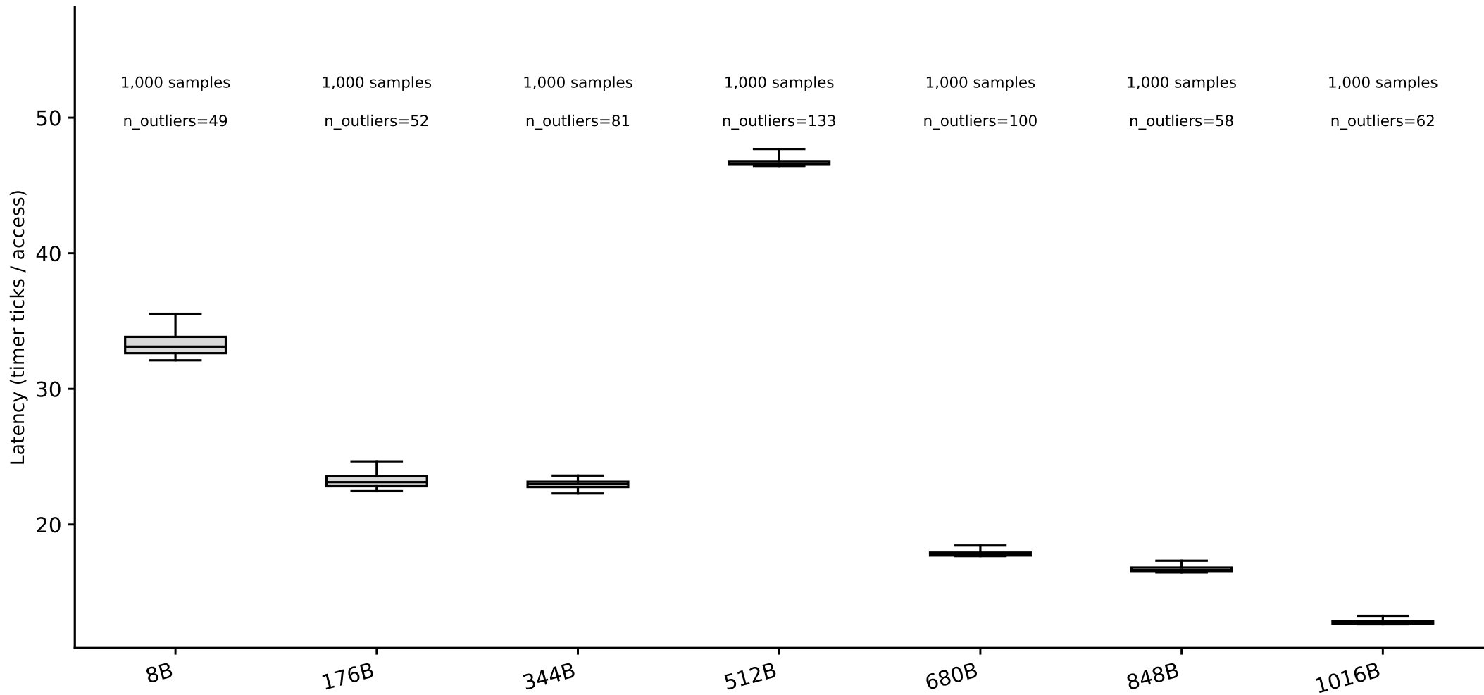
hazel_broadwell: line-size box plots, random pattern (whiskers = p5/p95) (Phase I timing-only, level boundary=262144B, single-curve method)
