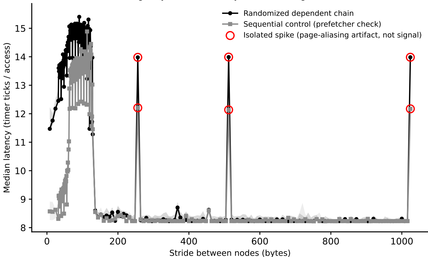
hazel_broadwell: line-size sweep (dependent pointer chase), footprint=64 KiB (Phase I timing-only, level boundary=32768B, single-curve method)
