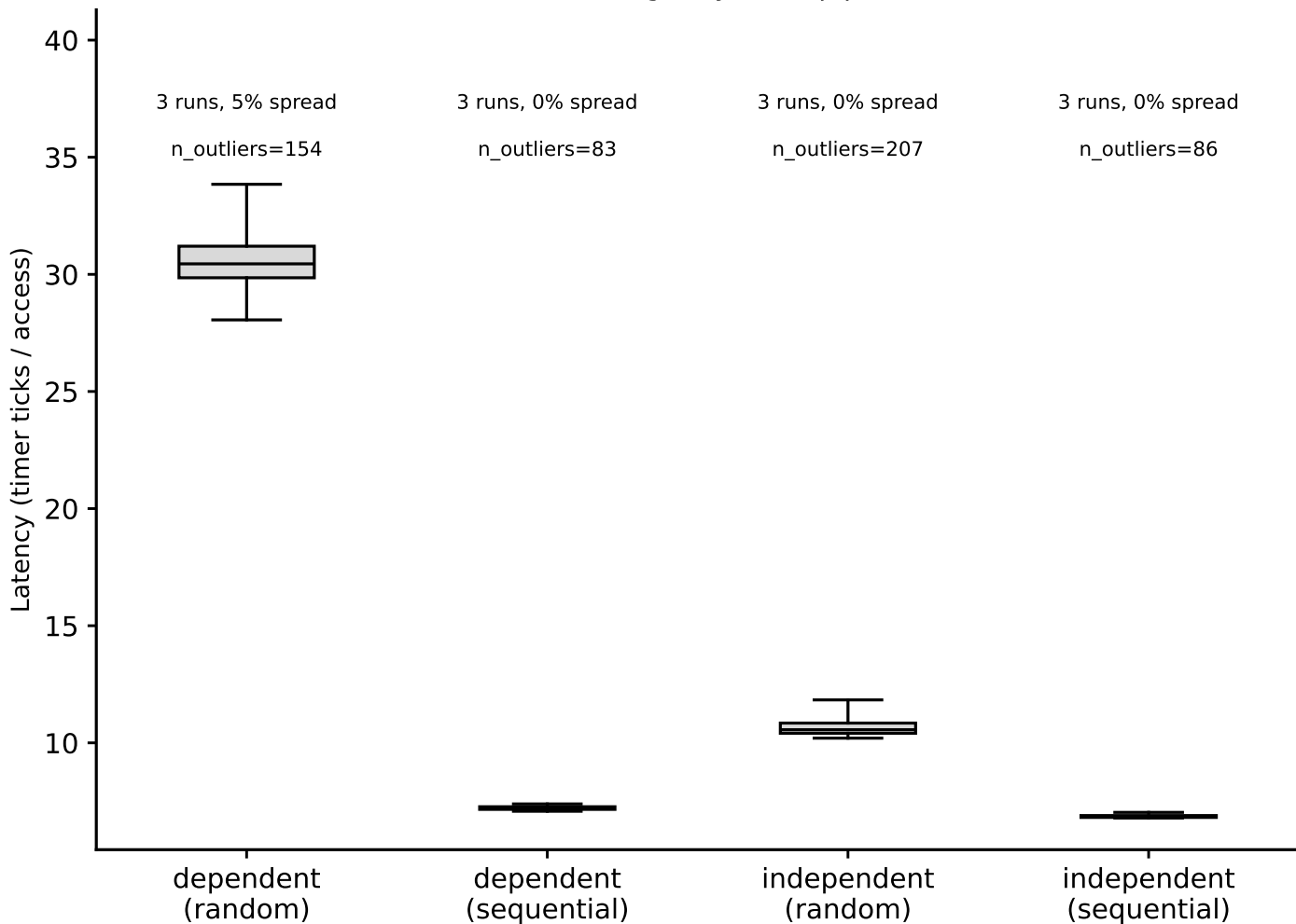
hazel_genoa: hit-latency box plots, L2 (footprint=1 MiB) (Phase I timing-only, auto pipeline)
