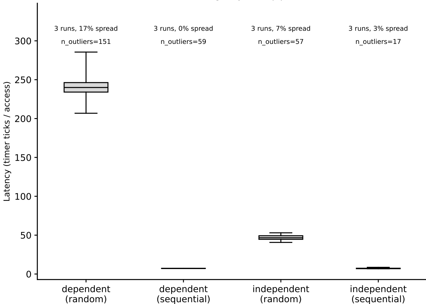
hazel_genoa: hit-latency box plots, LLC (footprint=32 MiB) (Phase I timing-only, auto pipeline)
