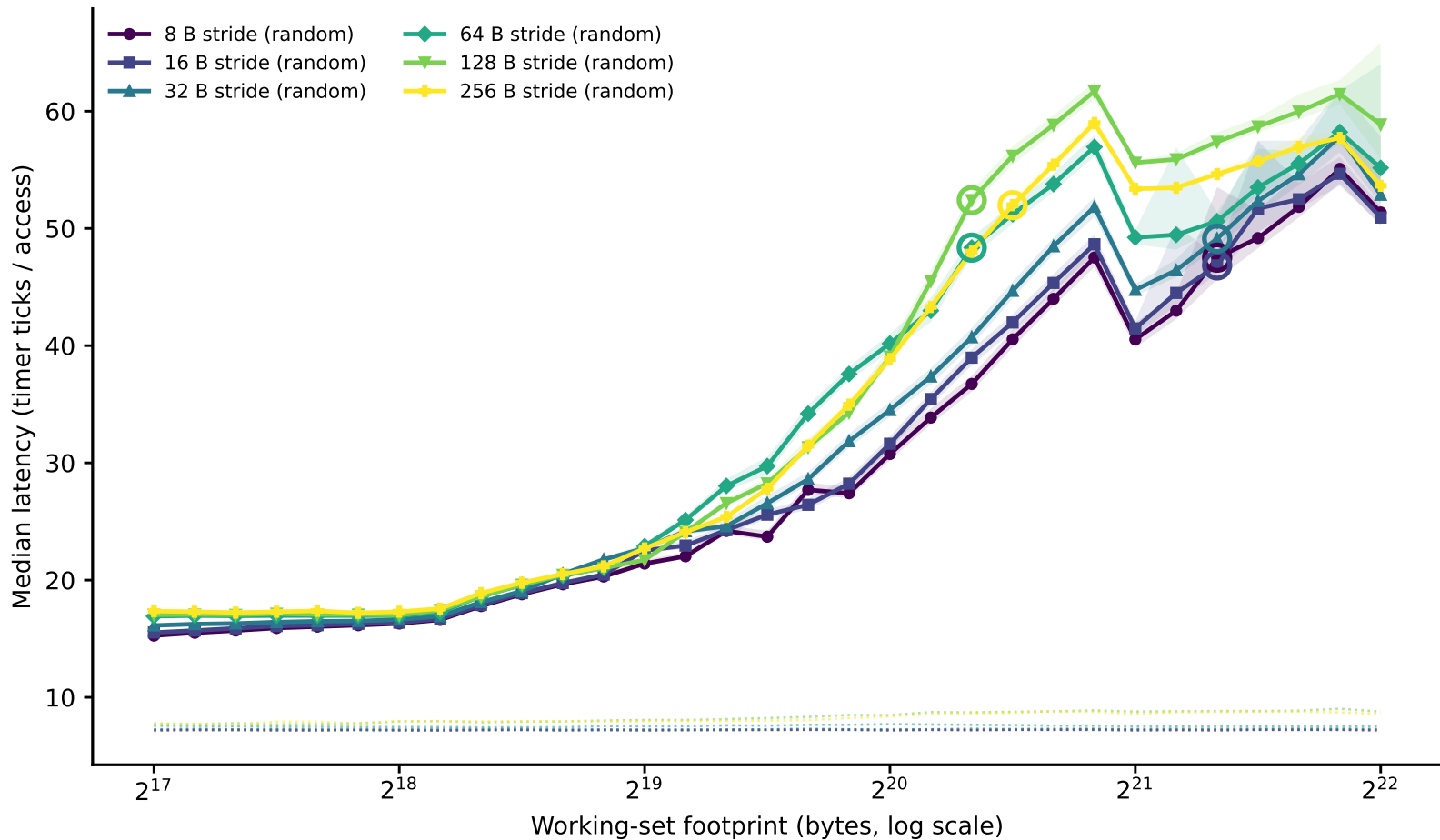
hazel_genoa: line-size family of curves (dependent pointer chase) (Phase I timing-only, level boundary=1048576B window=[131072,4194304])
