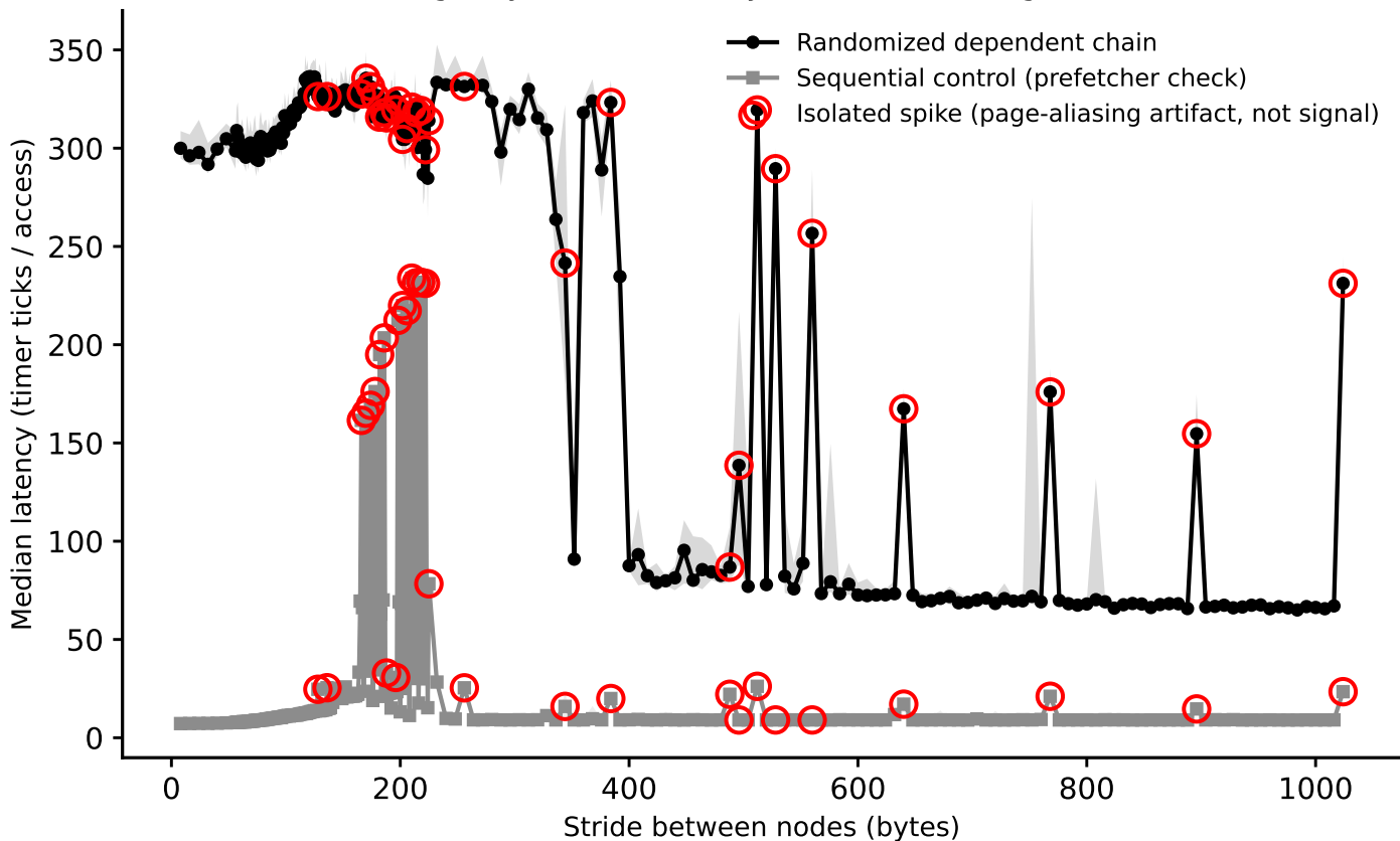
hazel_genoa: line-size sweep (dependent pointer chase), footprint=64 MiB (Phase I timing-only, level boundary=33554432B, single-curve method)
