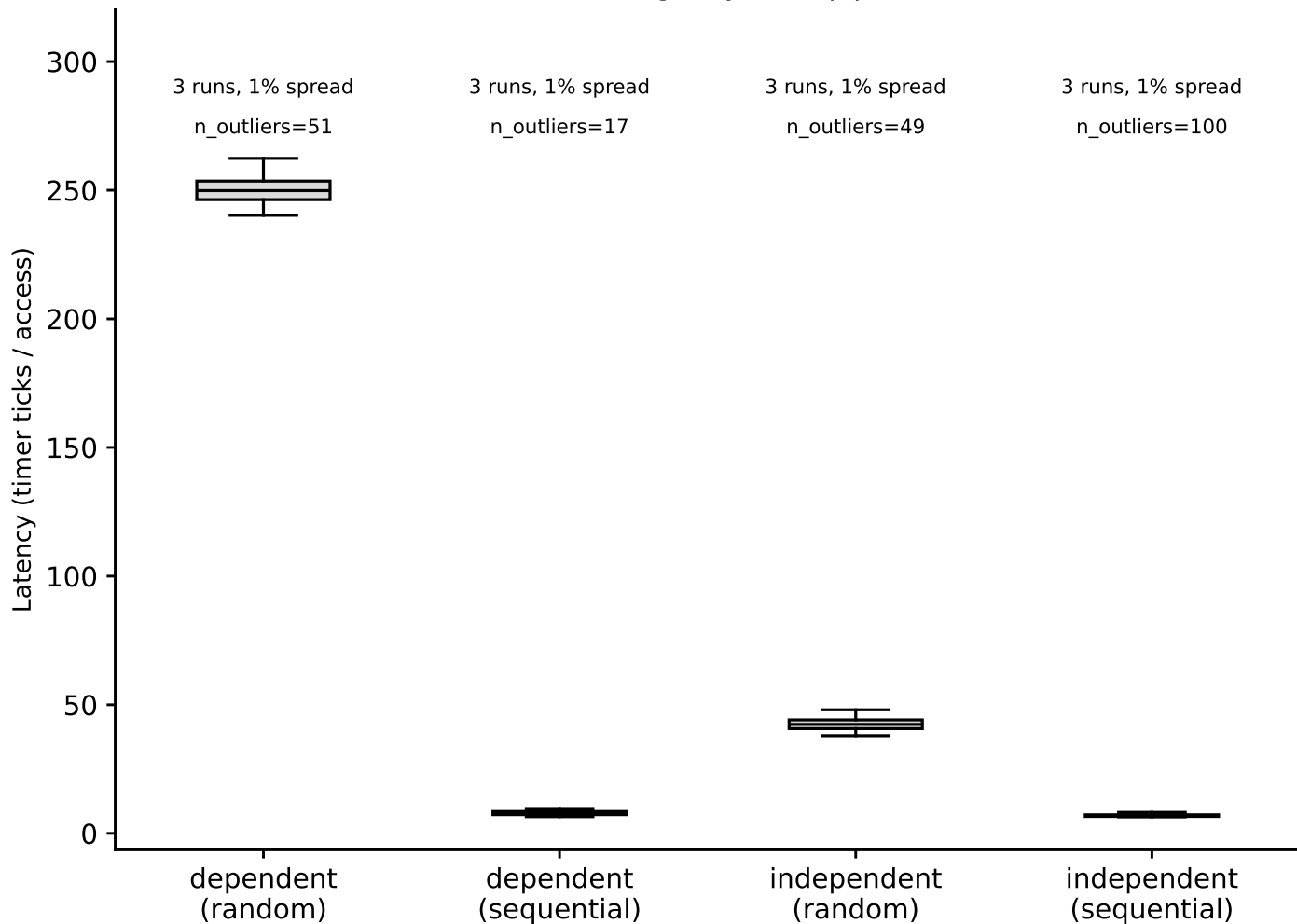
hazel_icelake_6326: hit-latency box plots, DRAM (footprint=512 MiB) (Phase I timing-only, auto pipeline)
