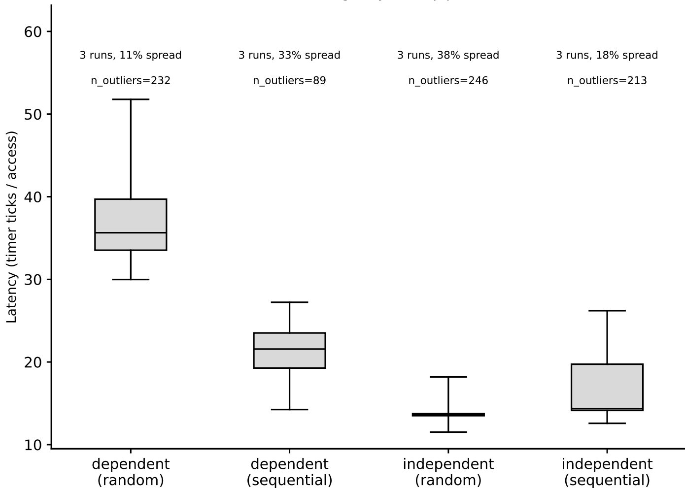
hazel_icelake_6326: hit-latency box plots, L2 (footprint=1.25 MiB) (Phase I timing-only, auto pipeline)
