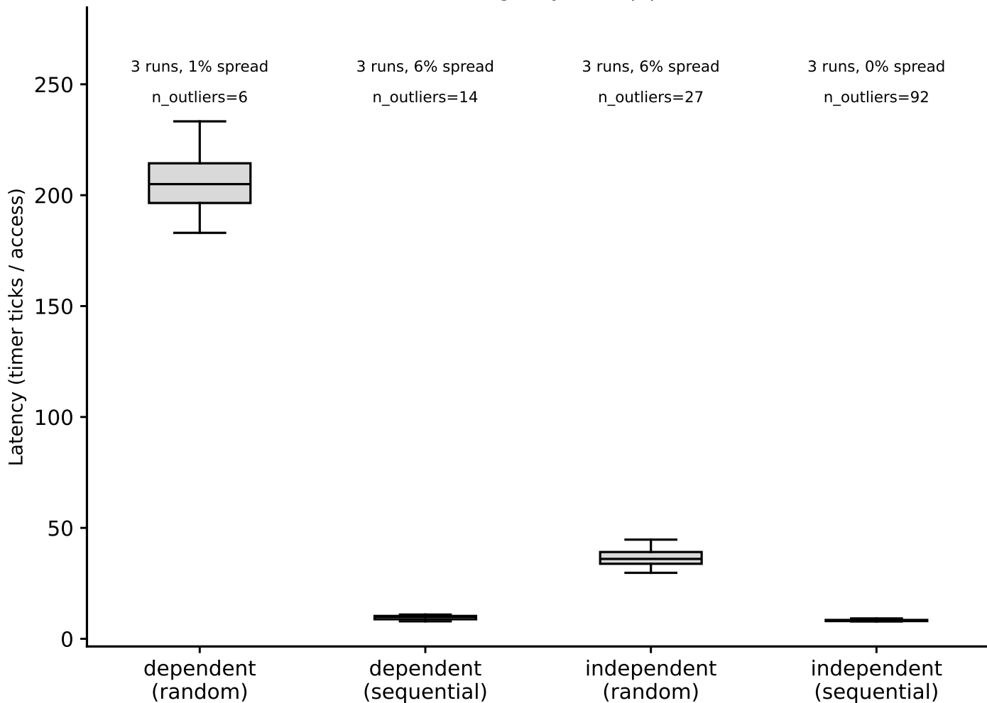
hazel_icelake_6326: hit-latency box plots, LLC (footprint=24.6754 MiB) (Phase I timing-only, auto pipeline)
