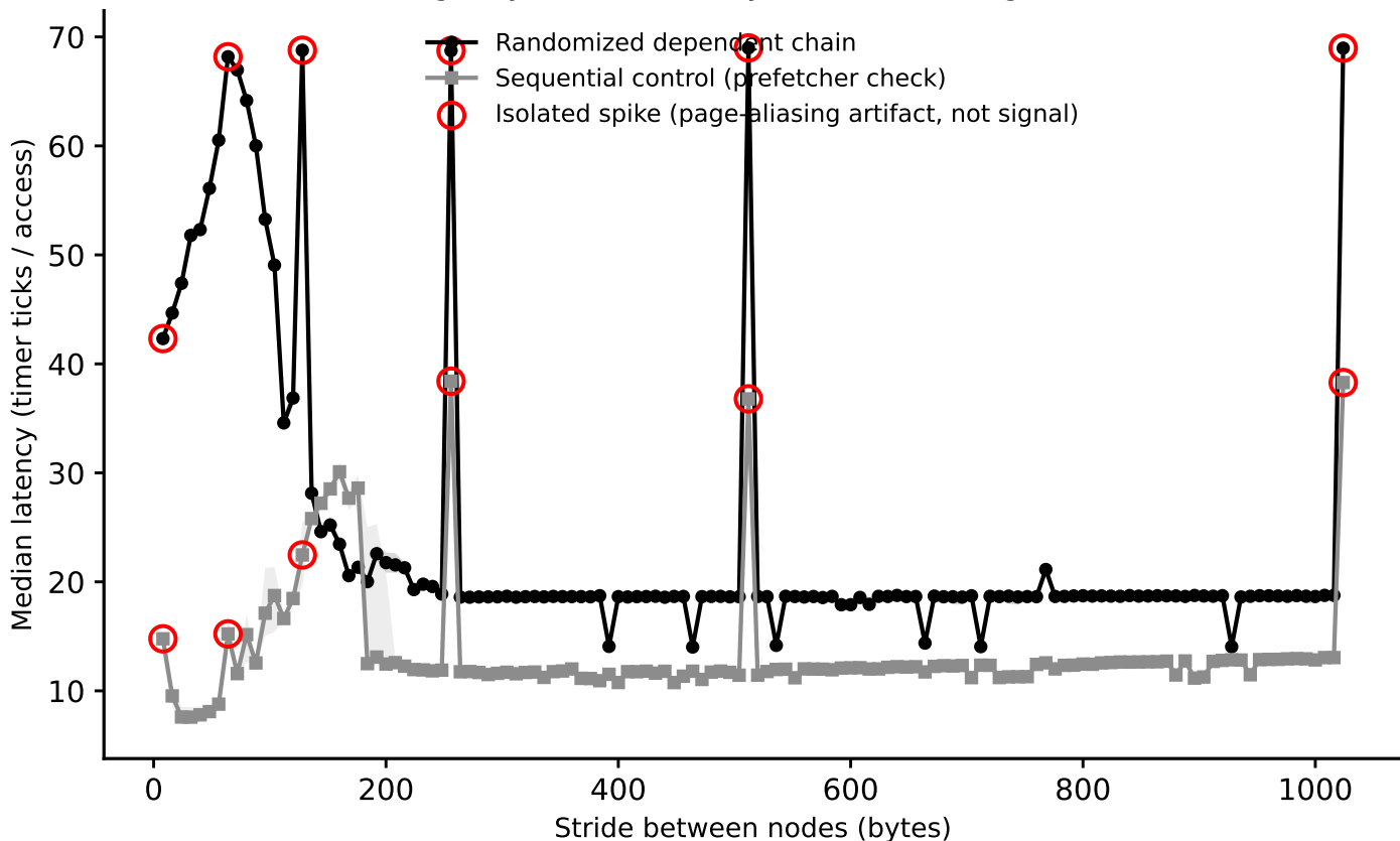
hazel_icelake_6326: line-size sweep (dependent pointer chase), footprint=2.5 MiB (Phase I timing-only, level boundary=1310720B, single-curve method)
