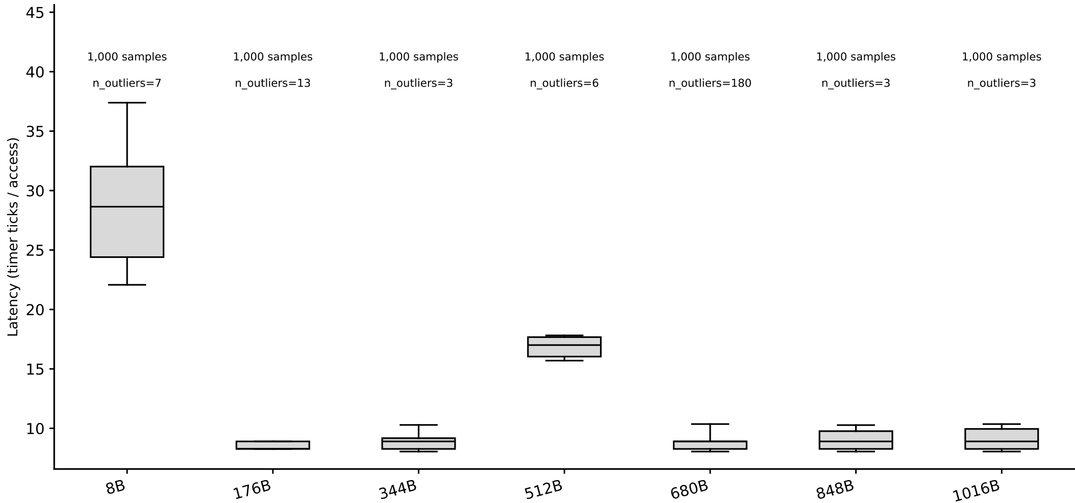
hazel_icelake_6326: line-size box plots, random pattern (whiskers = p5/p95) (Phase I timing-only, level boundary=32768B, single-curve method)
