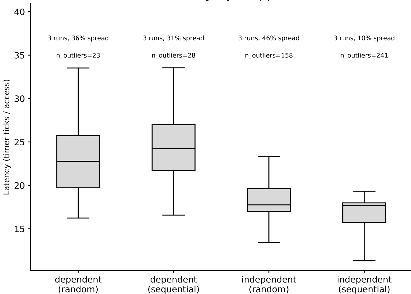
hazel_icelake_8358: hit-latency box plots, L1 (footprint=32 KiB) (Phase I timing-only, auto pipeline)
