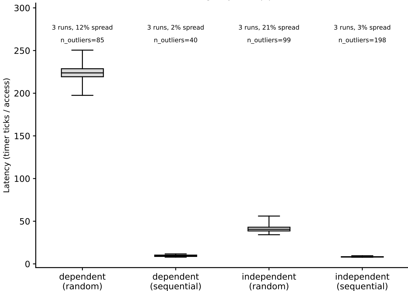
hazel_icelake_8358: hit-latency box plots, LLC (footprint=48 MiB) (Phase I timing-only, auto pipeline)
