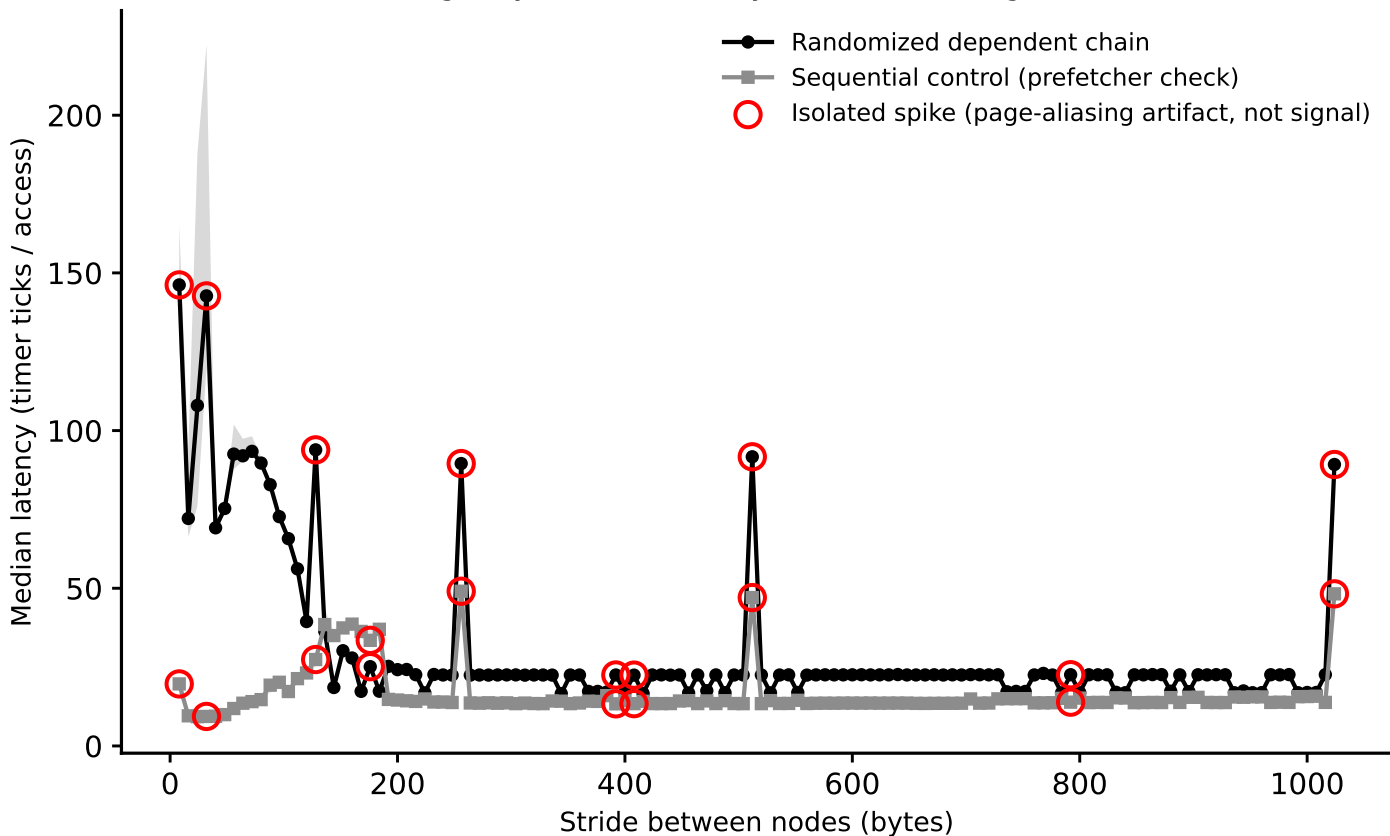
hazel_icelake_8358: line-size sweep (dependent pointer chase), footprint=2.5 MiB (Phase I timing-only, level boundary=1310720B, single-curve method)
