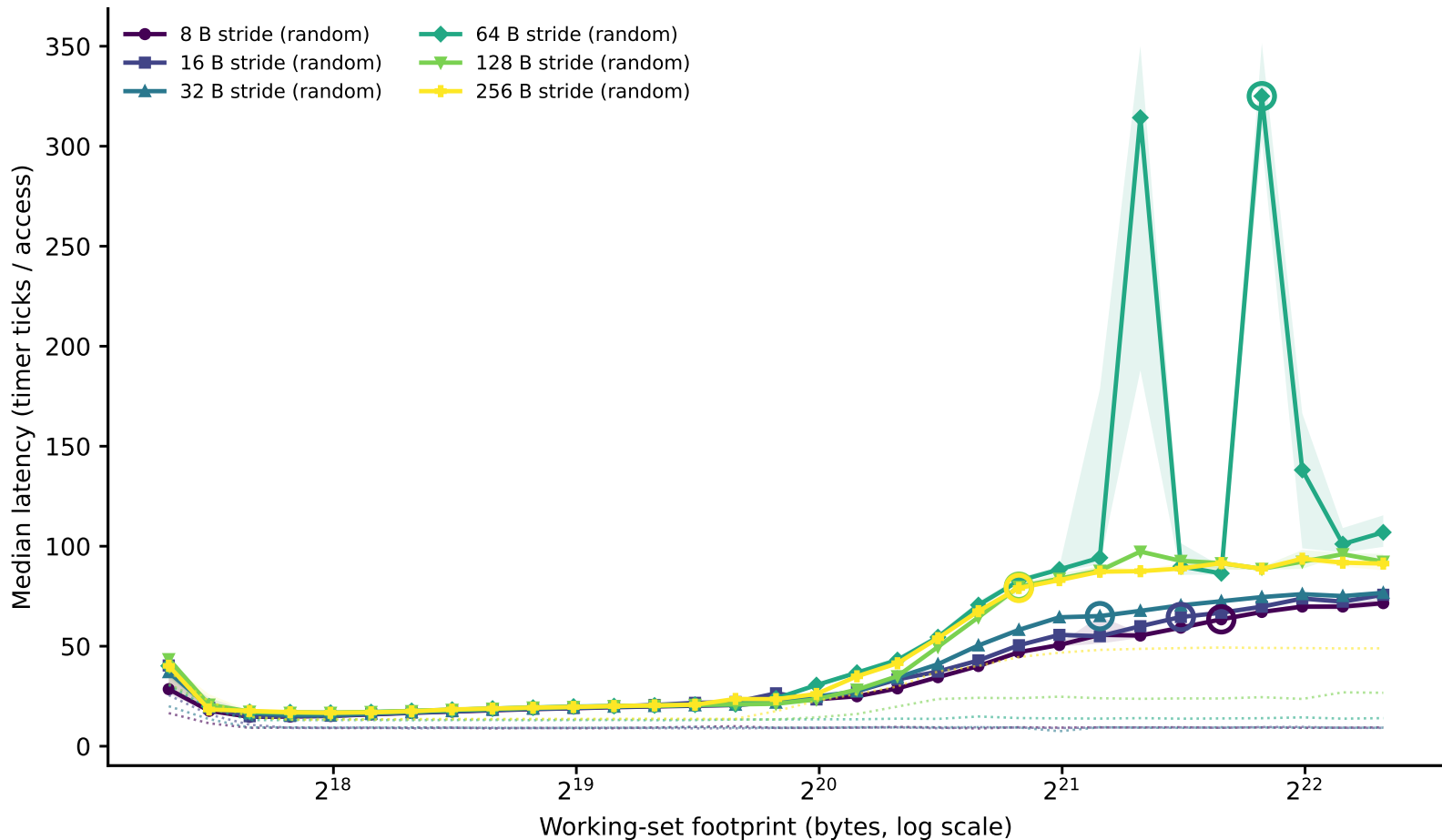
hazel_icelake_8358: line-size family of curves (dependent pointer chase) (Phase I timing-only, level boundary=1310720B window=[163840,5242880])
