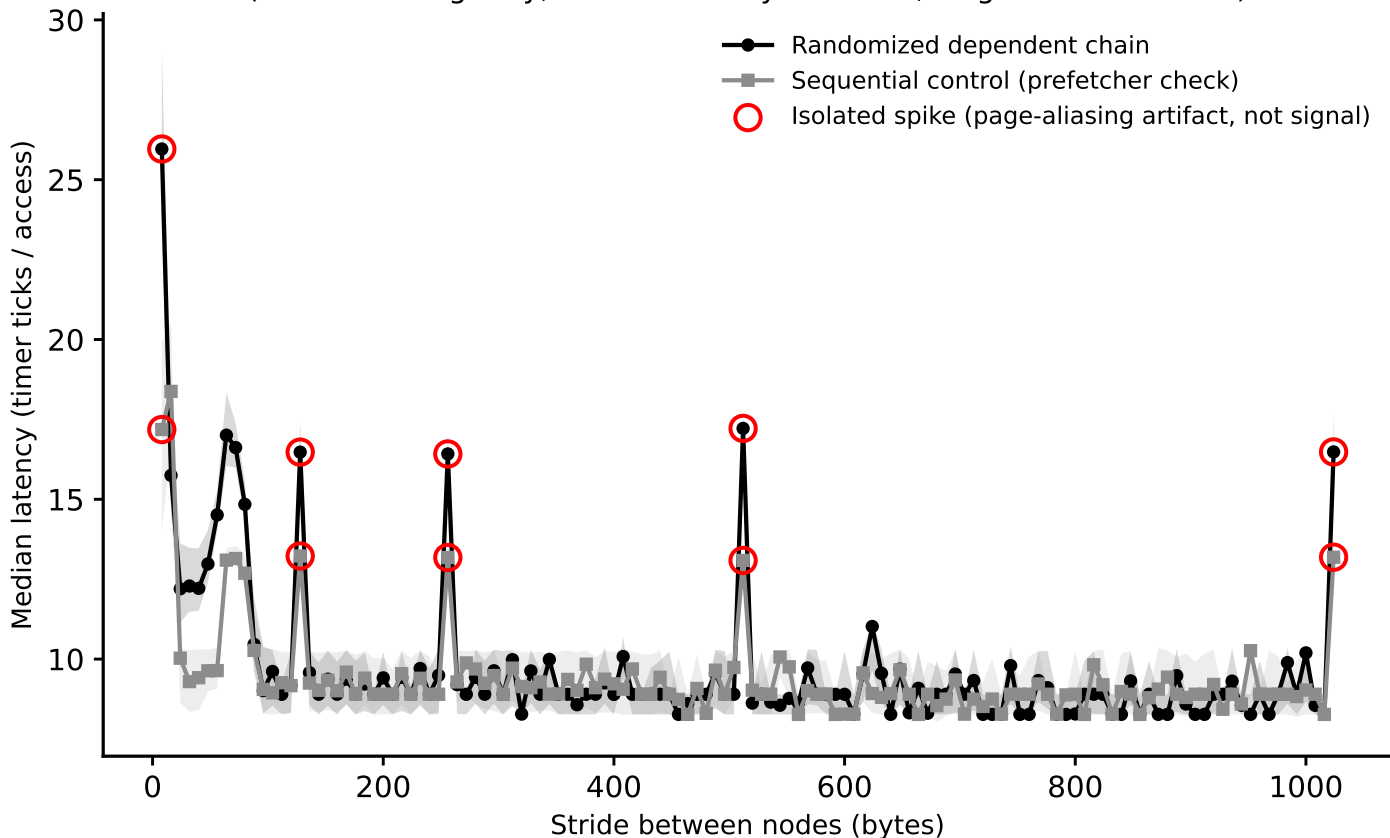
hazel_icelake_8358: line-size sweep (dependent pointer chase), footprint=64 KiB (Phase I timing-only, level boundary=32768B, single-curve method)
