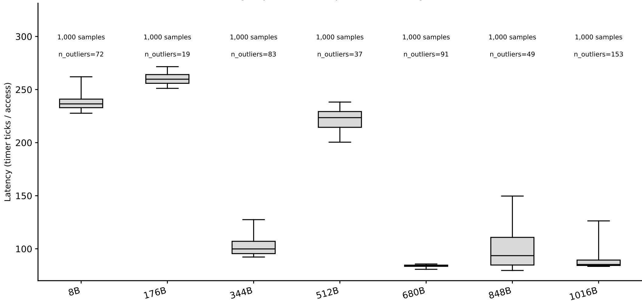
hazel_icelake_8358: line-size box plots, random pattern (whiskers = p5/p95) (Phase I timing-only, level boundary=50331648B, single-curve method)
