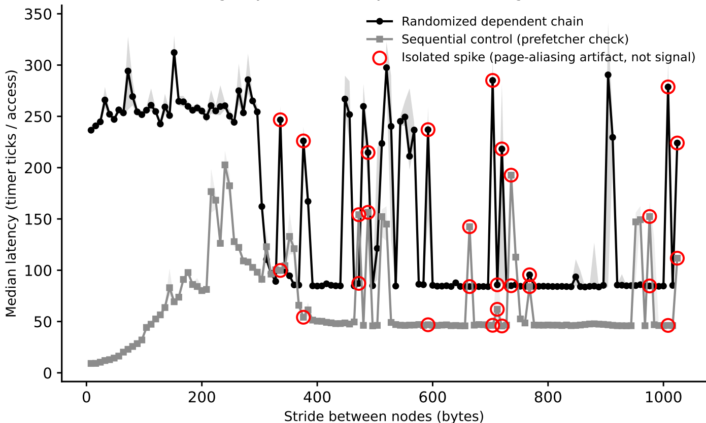
hazel_icelake_8358: line-size sweep (dependent pointer chase), footprint=96 MiB (Phase I timing-only, level boundary=50331648B, single-curve method)
